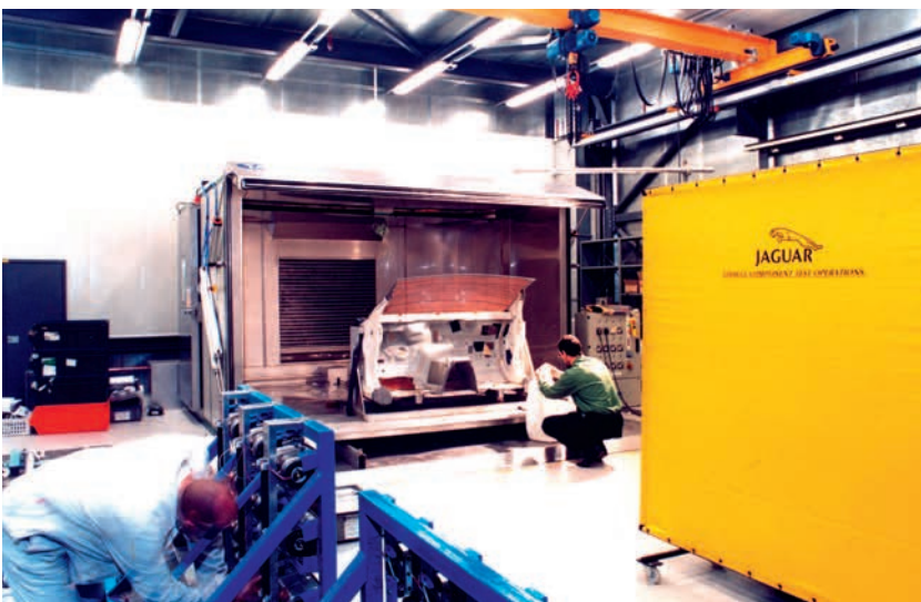
Airbag in-vehicle testing chamber, Jaguar, UK
